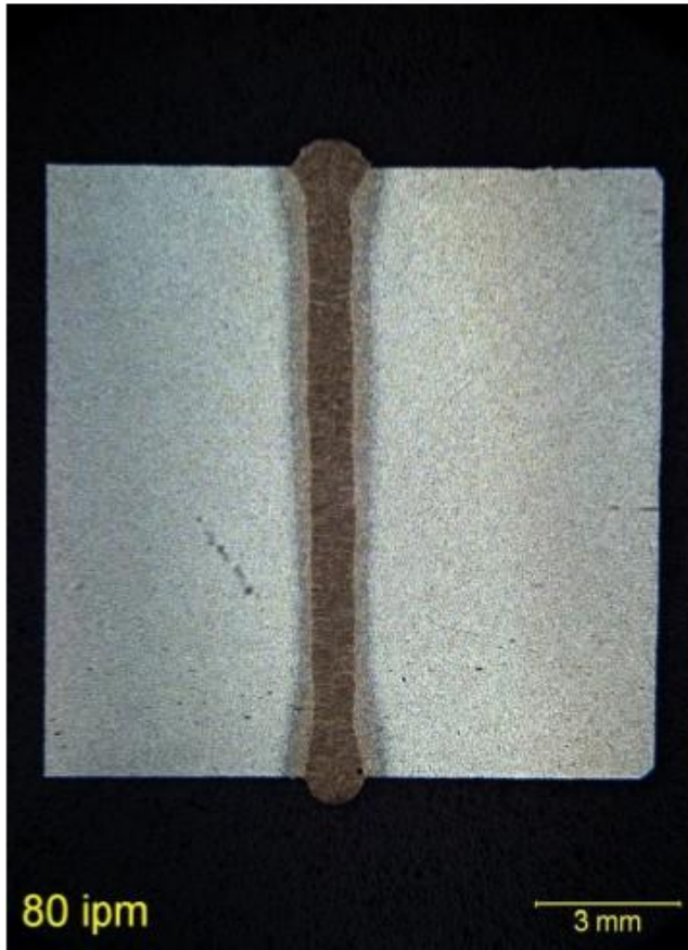
14 mm S.S 10 kW compliments EWI Columbus Ohio
